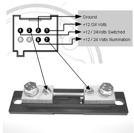
Required Viewline 60mv Shunt Recommend 10 AWG wire from Shunt
