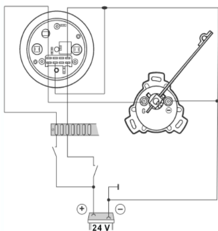
Single Station 24V
