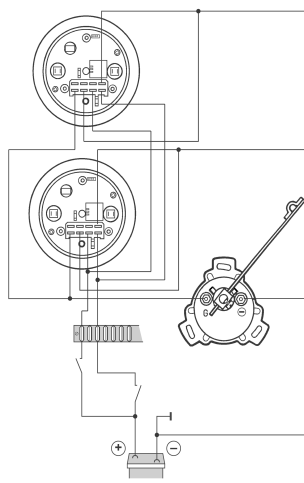
Dual Station 24V
