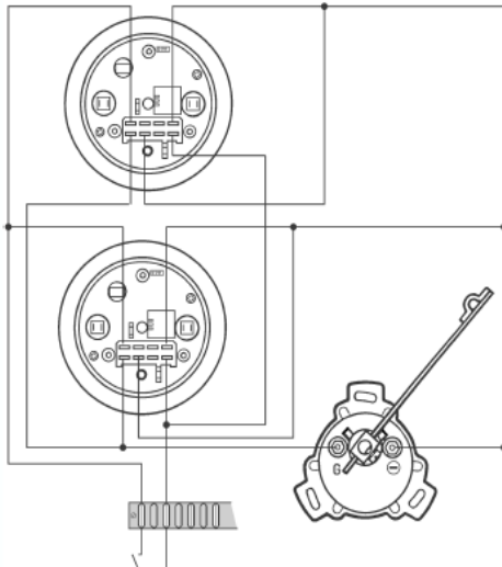
Dual Station 24V
